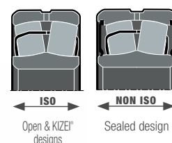
Spherical roller bearing
